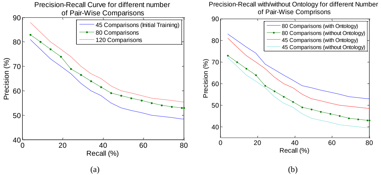
Figure 44: The effect of the number of selected samples on the precision-recall curve. (a) Precision recall for different numbers of comparisons (feedback iterations) as regards the proposed learning strategy. (b) The effect of ontology on precision-recall for different numbers of comparisons.
