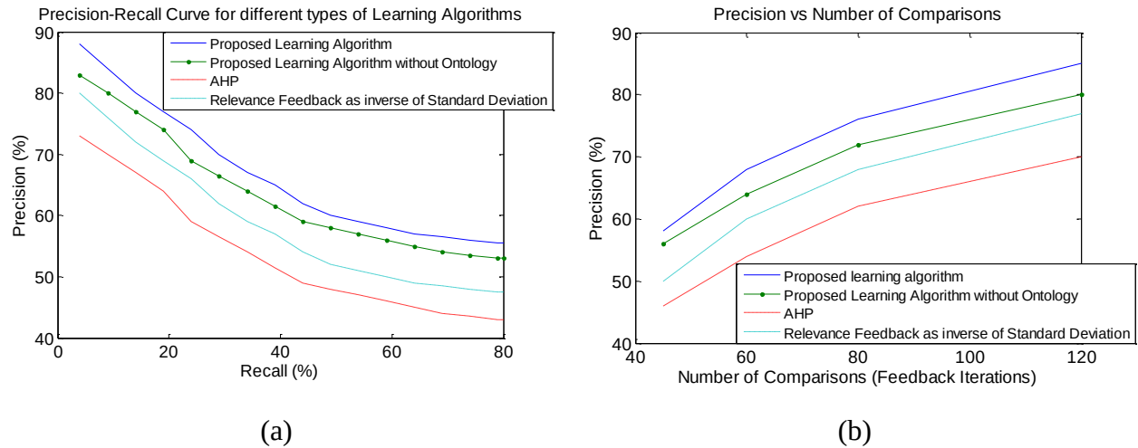
Figure 43: Comparisons of the proposed relevance feedback learning component with other online learning strategies and experimental documentation of the ontology driven rectification mechanism. (a) The precision-recall curve for various learning algorithms versus the proposed one. (b) The precision versus the number of feedback iterations to illustrate the effect of number of pairwise comparisons on the overall system performance. The results have been obtained at recall 50%.
